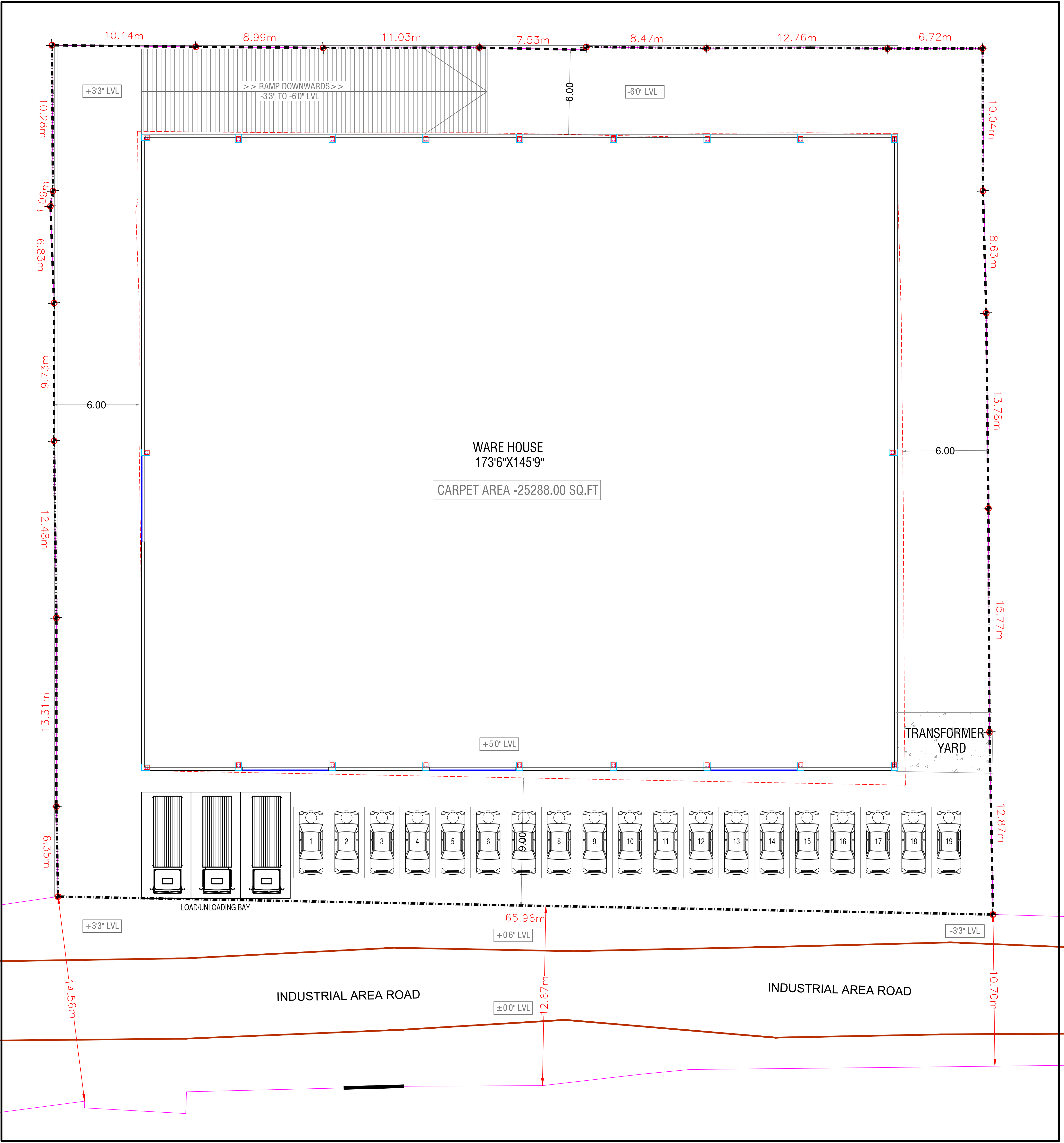
GROUND FLOOR PLAN PRELIMINARY SKETCH DESIGN PROPOSED WARE HOUSE AT BAIKAMPADY ,MANGALORE
